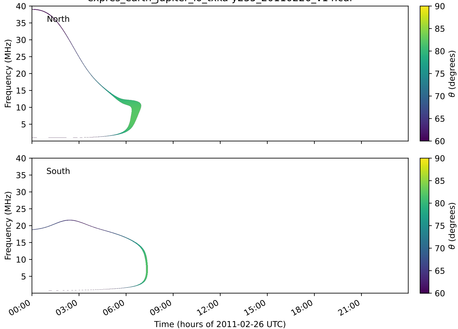
expres_earth_jupiter_io_txka-y235_20110226_v14.cdf
