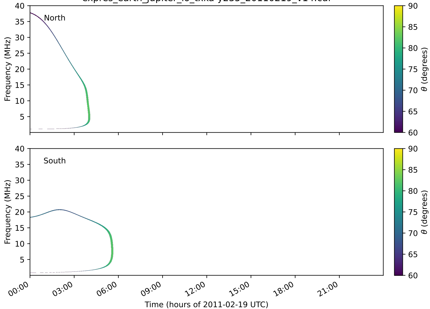
expres_earth_jupiter_io_txka-y235_20110219_v14.cdf
