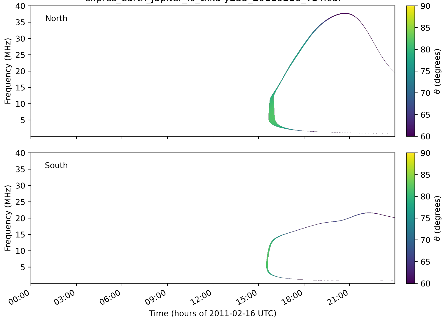
expres_earth_jupiter_io_txka-y235_20110216_v14.cdf
