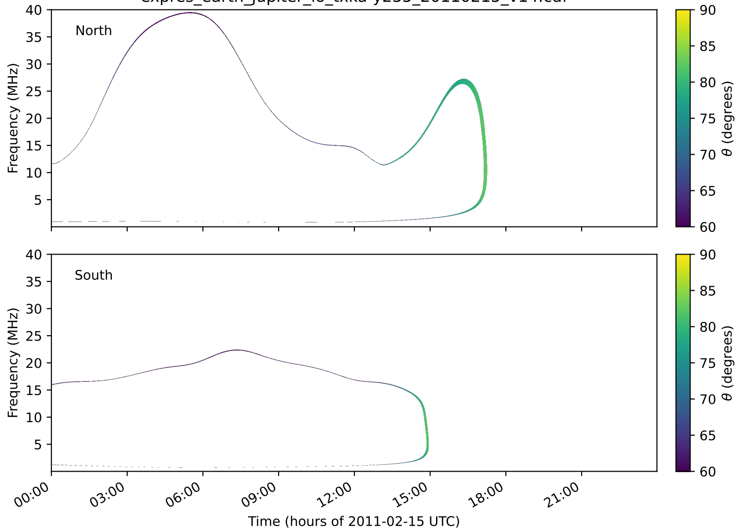
expres_earth_jupiter_io_txka-y235_20110215_v14.cdf
