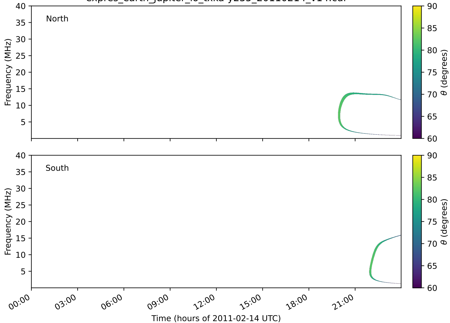
expres_earth_jupiter_io_txka-y235_20110214_v14.cdf
