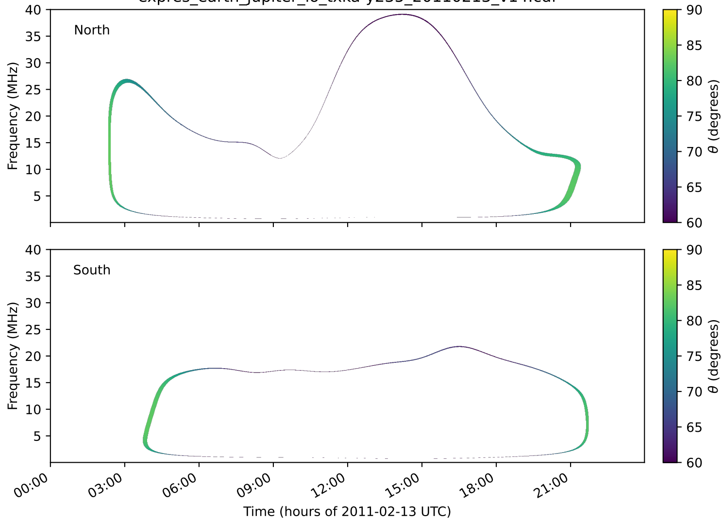
expres_earth_jupiter_io_txka-y235_20110213_v14.cdf
