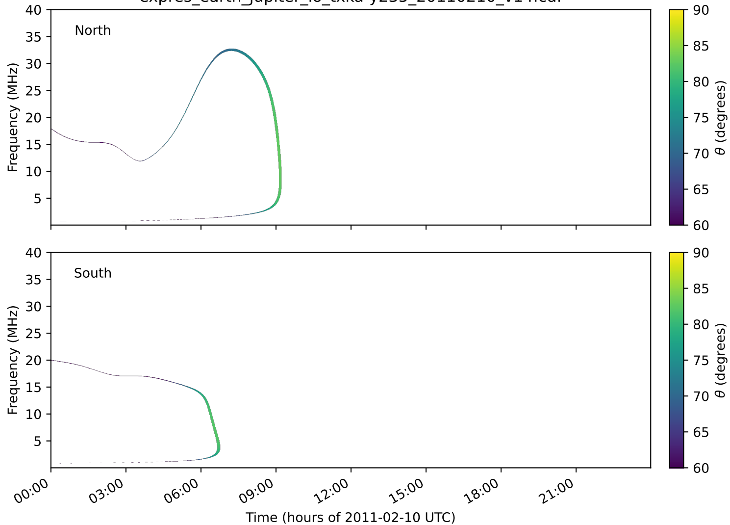
expres_earth_jupiter_io_txka-y235_20110210_v14.cdf
