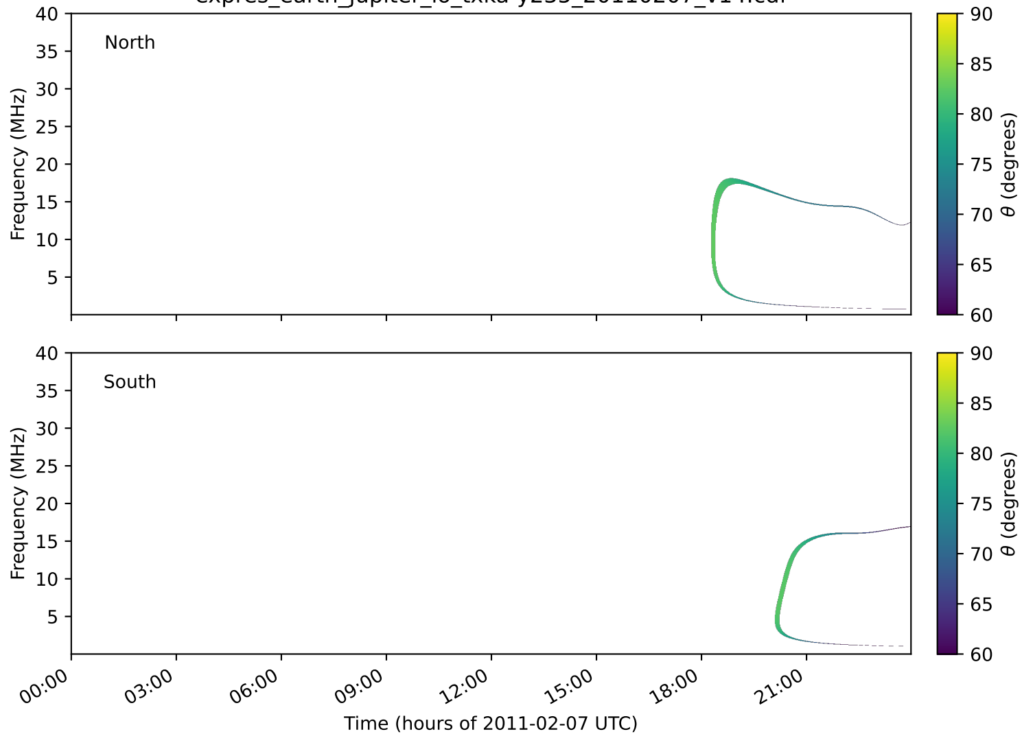
expres_earth_jupiter_io_txka-y235_20110207_v14.cdf
