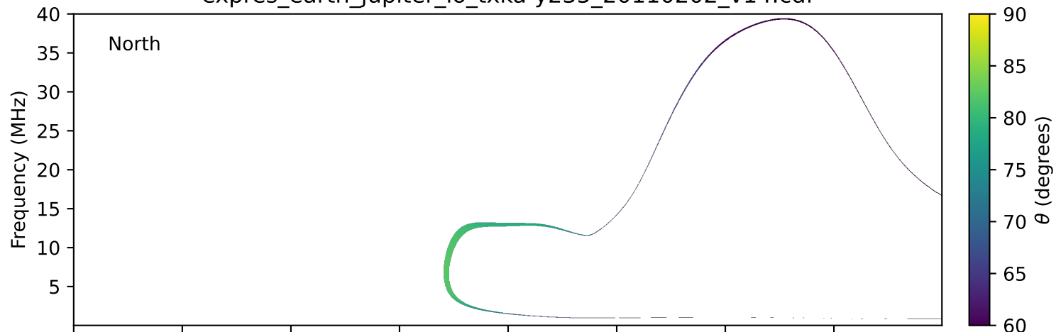
expres_earth_jupiter_io_txka-y235_20110202_v14.cdf
