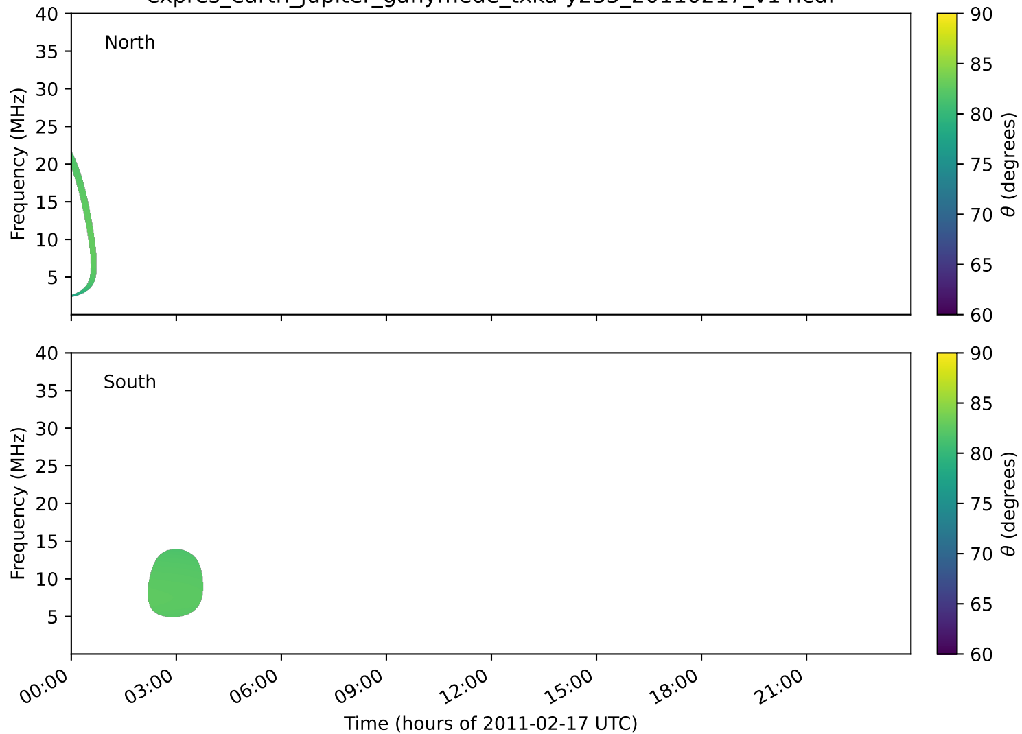
expres_earth_jupiter_ganymede_txka-y235_20110217_v14.cdf
