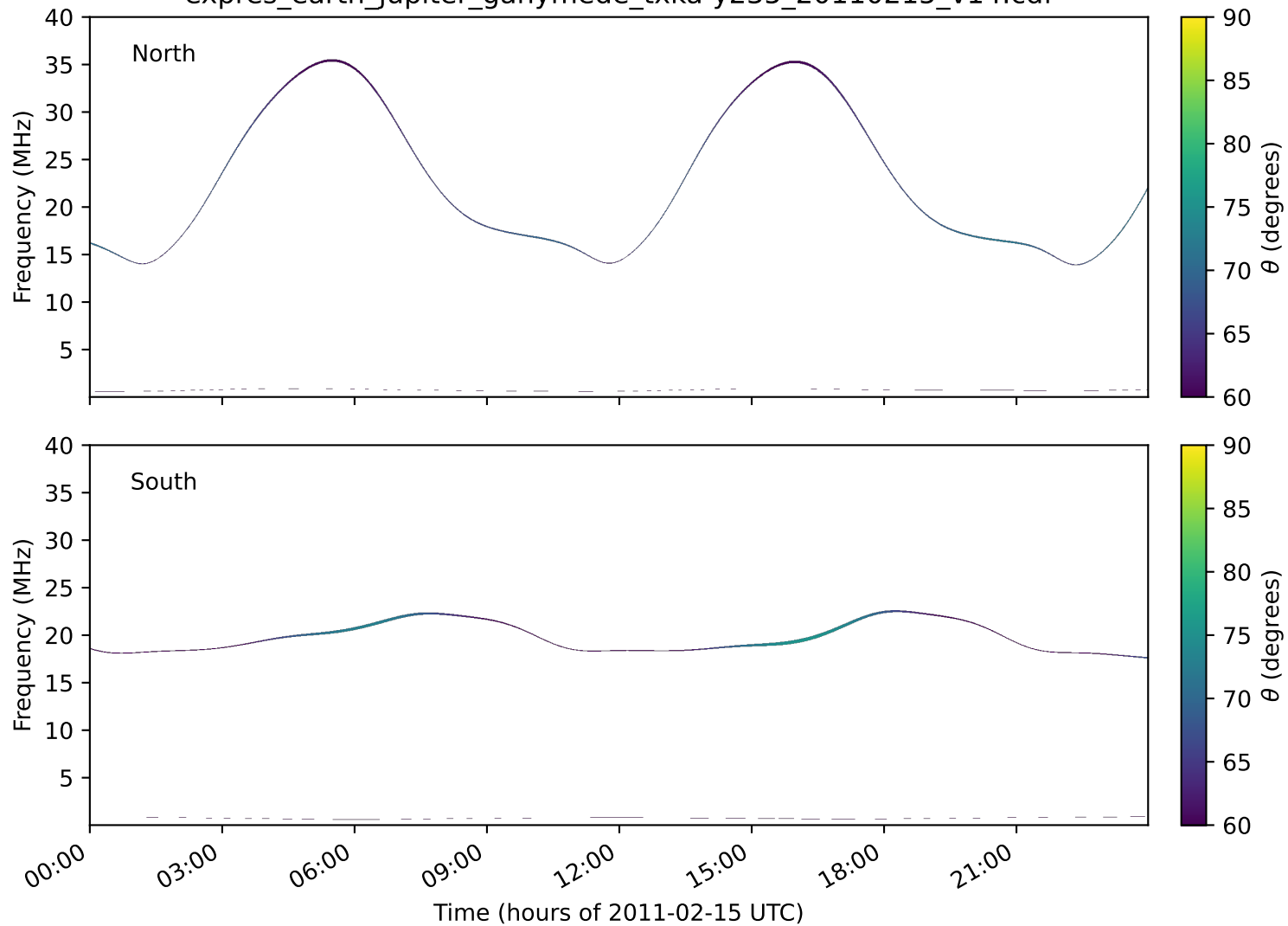
expres_earth_jupiter_ganymede_txka-y235_20110215_v14.cdf
