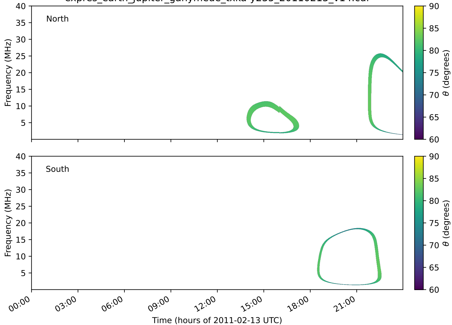
expres_earth_jupiter_ganymede_txka-y235_20110213_v14.cdf
