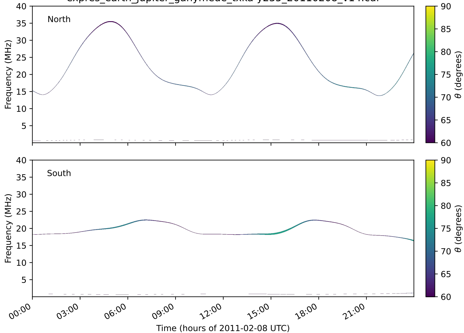
expres_earth_jupiter_ganymede_txka-y235_20110208_v14.cdf
