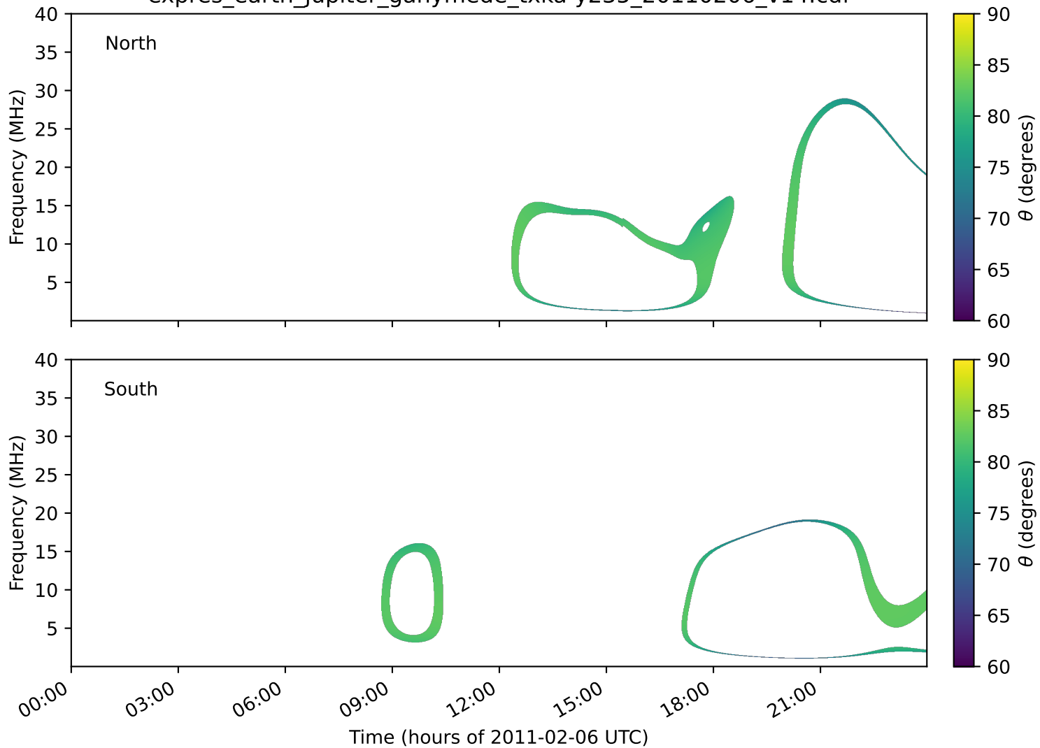
expres_earth_jupiter_ganymede_txka-y235_20110206_v14.cdf
