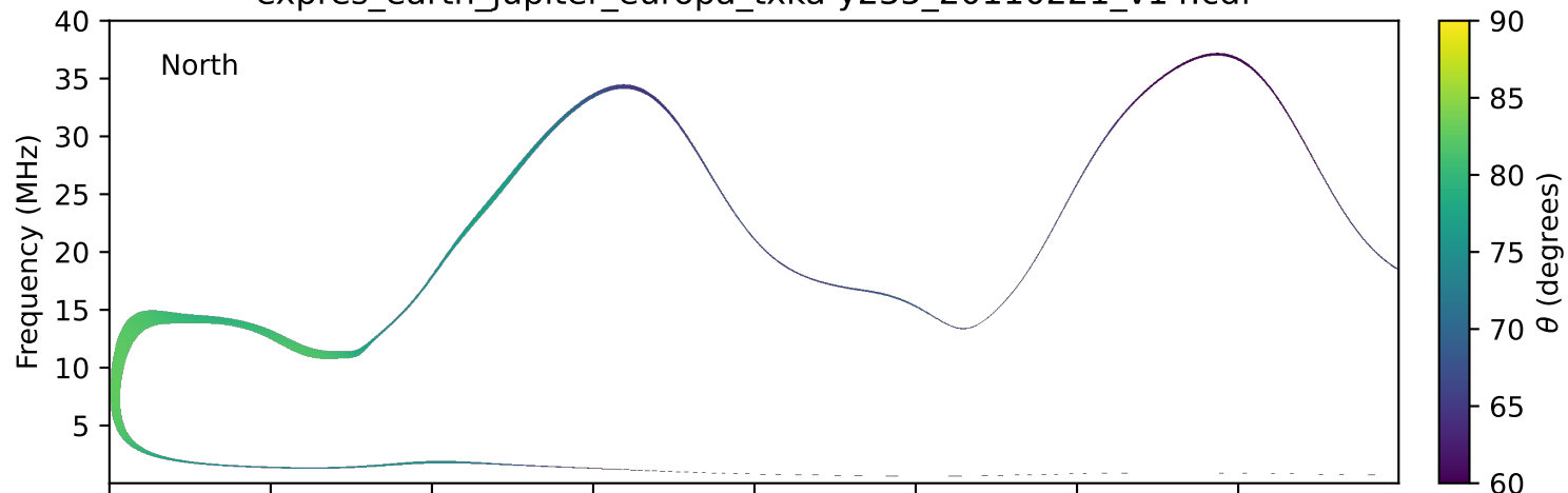
expres_earth_jupiter_europa_txka-y235_20110221_v14.cdf
