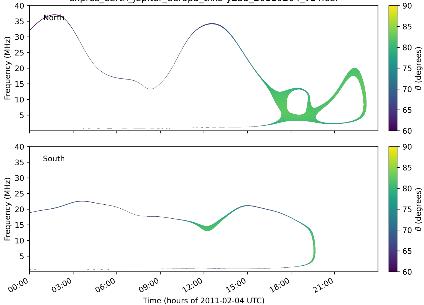
expres_earth_jupiter_europa_txka-y235_20110204_v14.cdf
