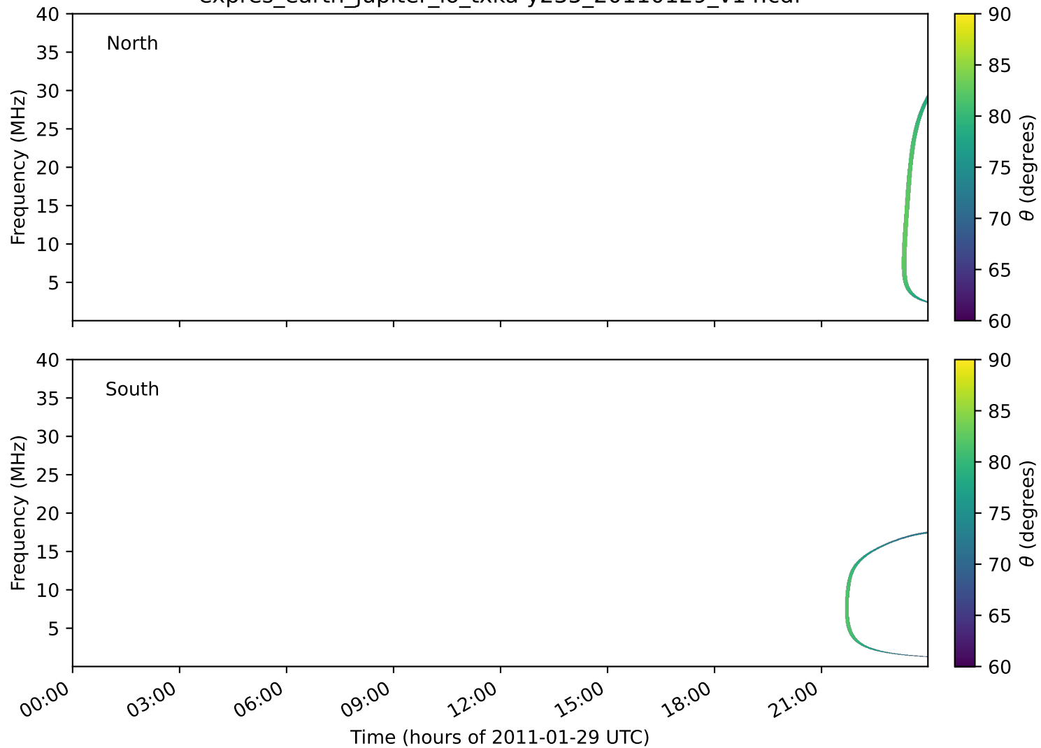
expres_earth_jupiter_io_txka-y235_20110129_v14.cdf
