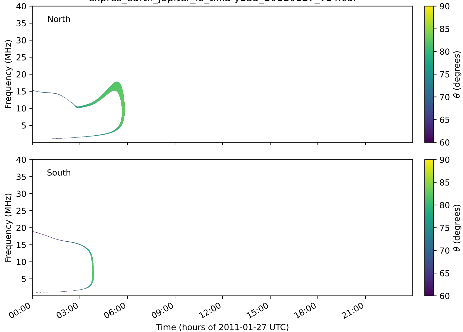
expres_earth_jupiter_io_txka-y235_20110127_v14.cdf
