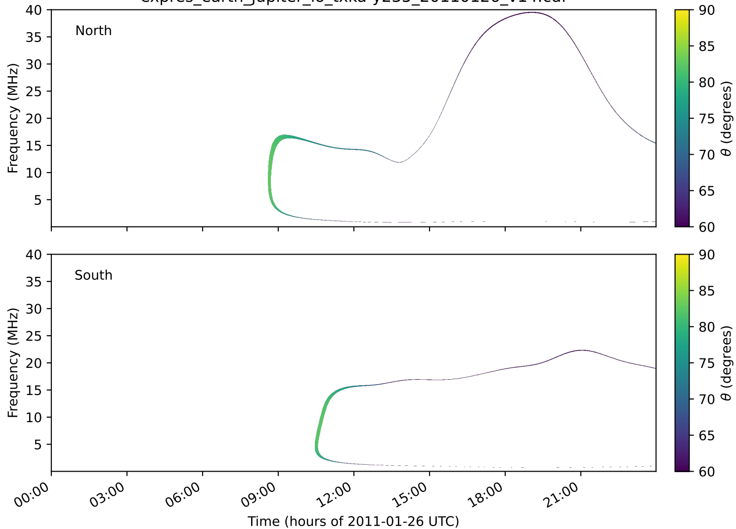
expres_earth_jupiter_io_txka-y235_20110126_v14.cdf
