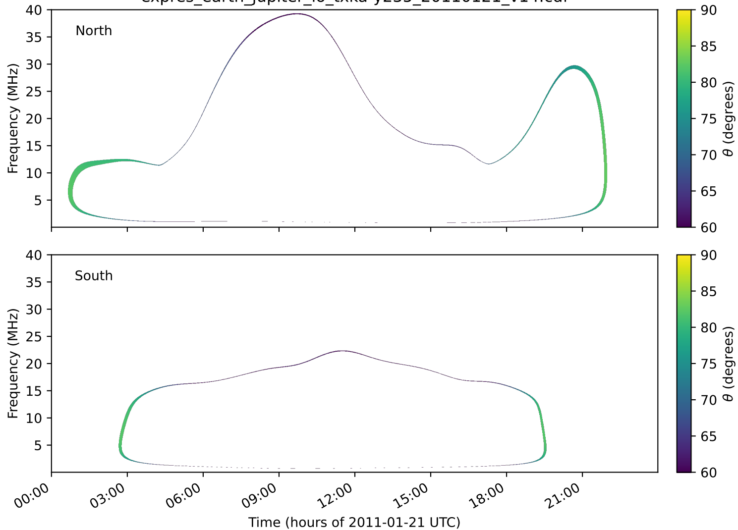
expres_earth_jupiter_io_txka-y235_20110121_v14.cdf
