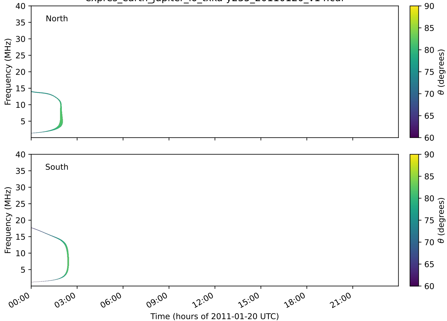
expres_earth_jupiter_io_txka-y235_20110120_v14.cdf
