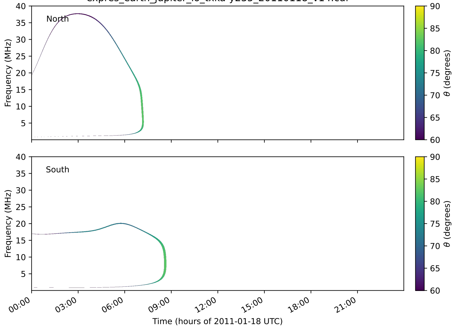
expres_earth_jupiter_io_txka-y235_20110118_v14.cdf
