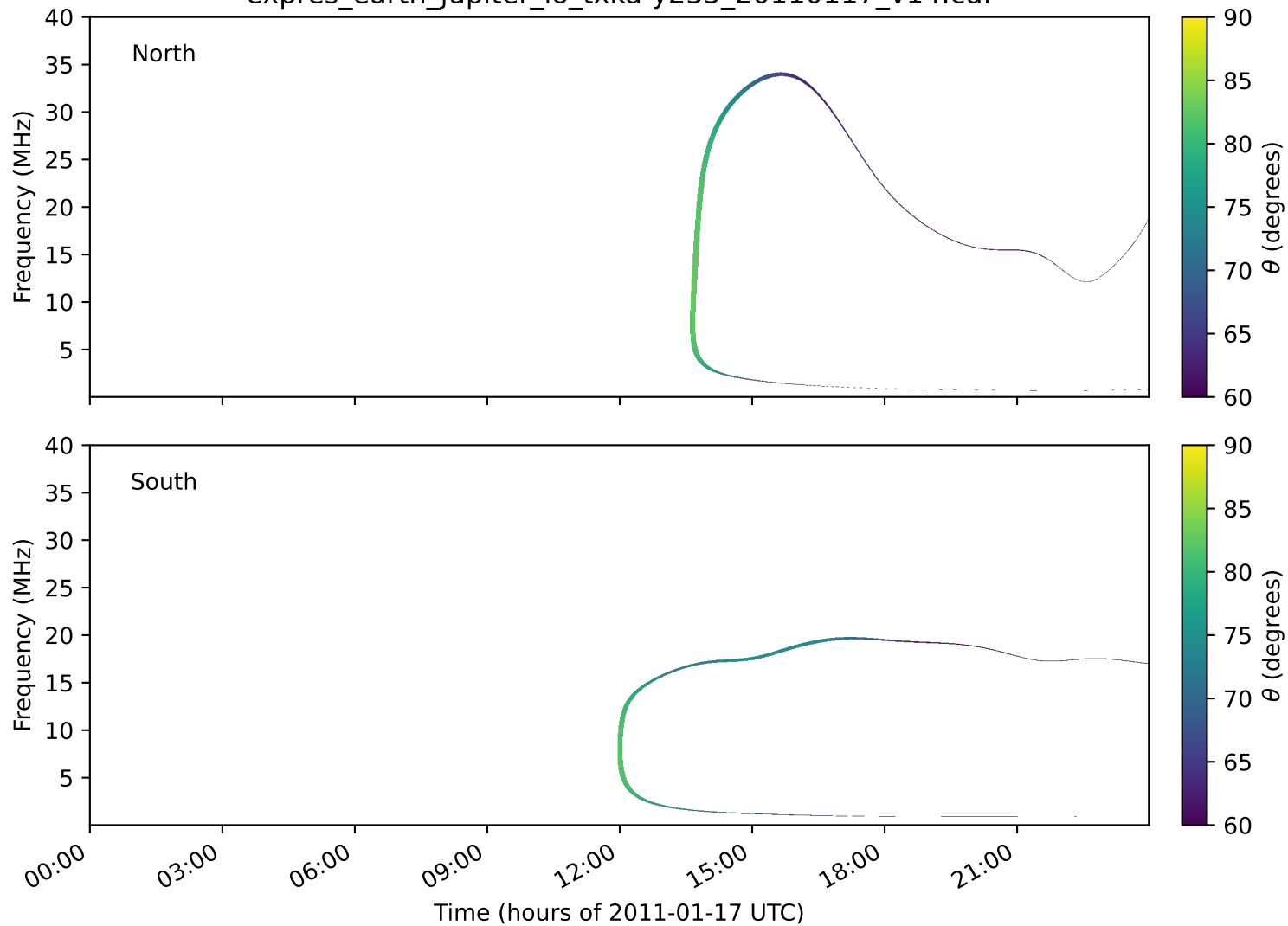
expres_earth_jupiter_io_txka-y235_20110117_v14.cdf
