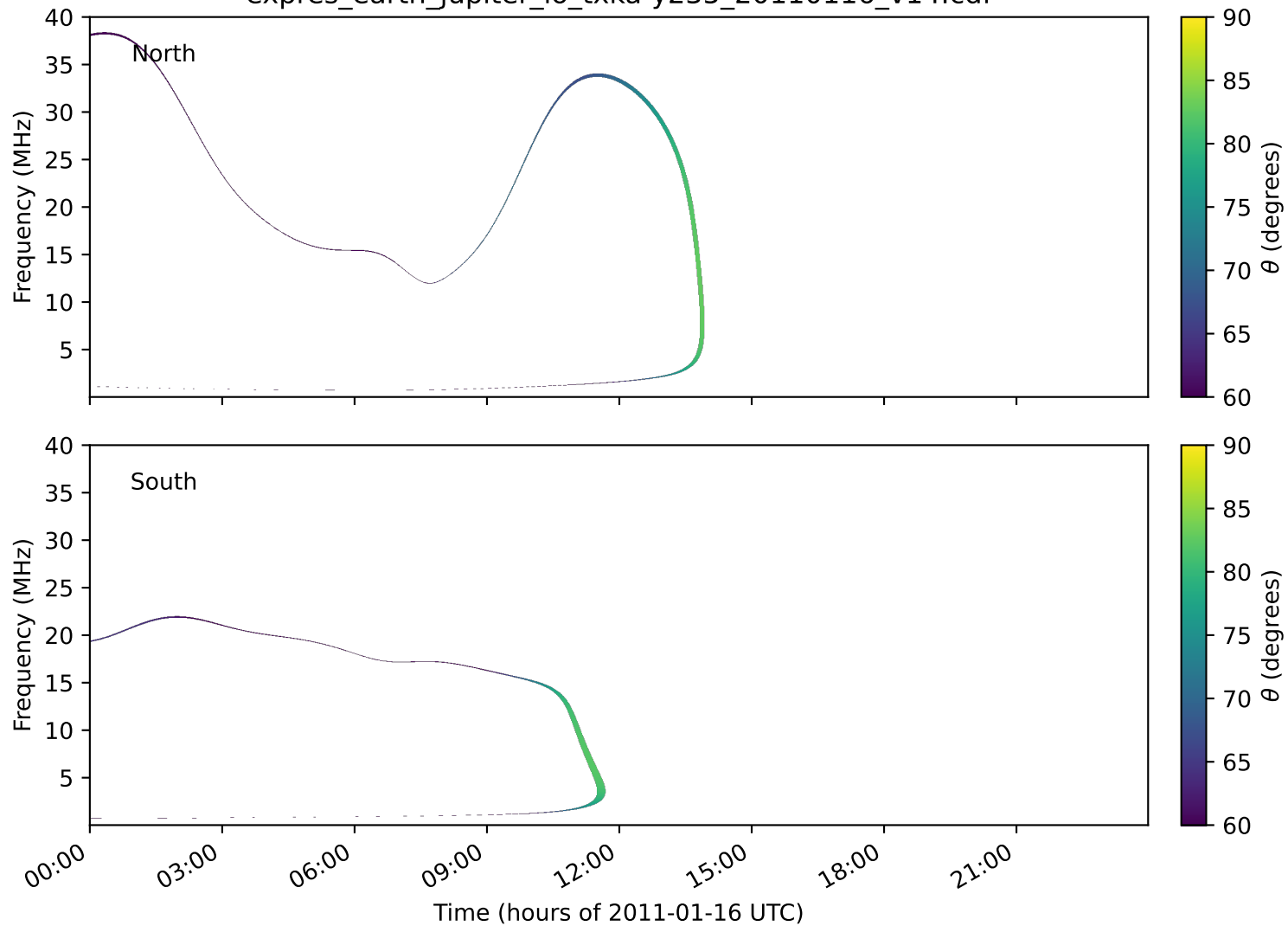
expres_earth_jupiter_io_txka-y235_20110116_v14.cdf
