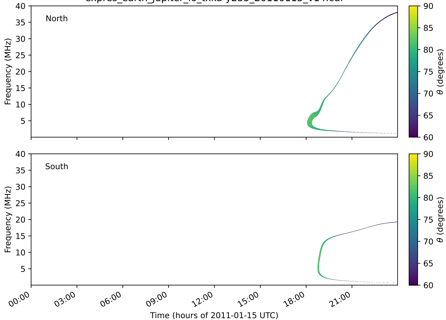
expres_earth_jupiter_io_txka-y235_20110115_v14.cdf
