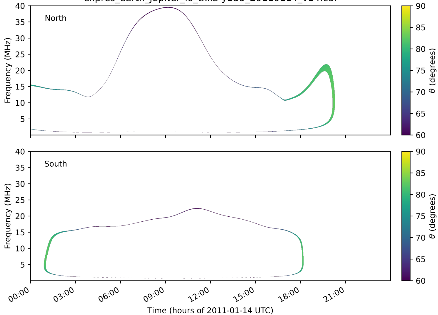
expres_earth_jupiter_io_txka-y235_20110114_v14.cdf
