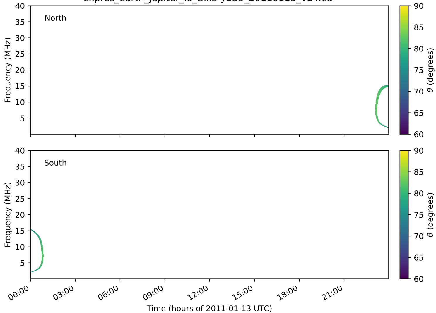
expres_earth_jupiter_io_txka-y235_20110113_v14.cdf
