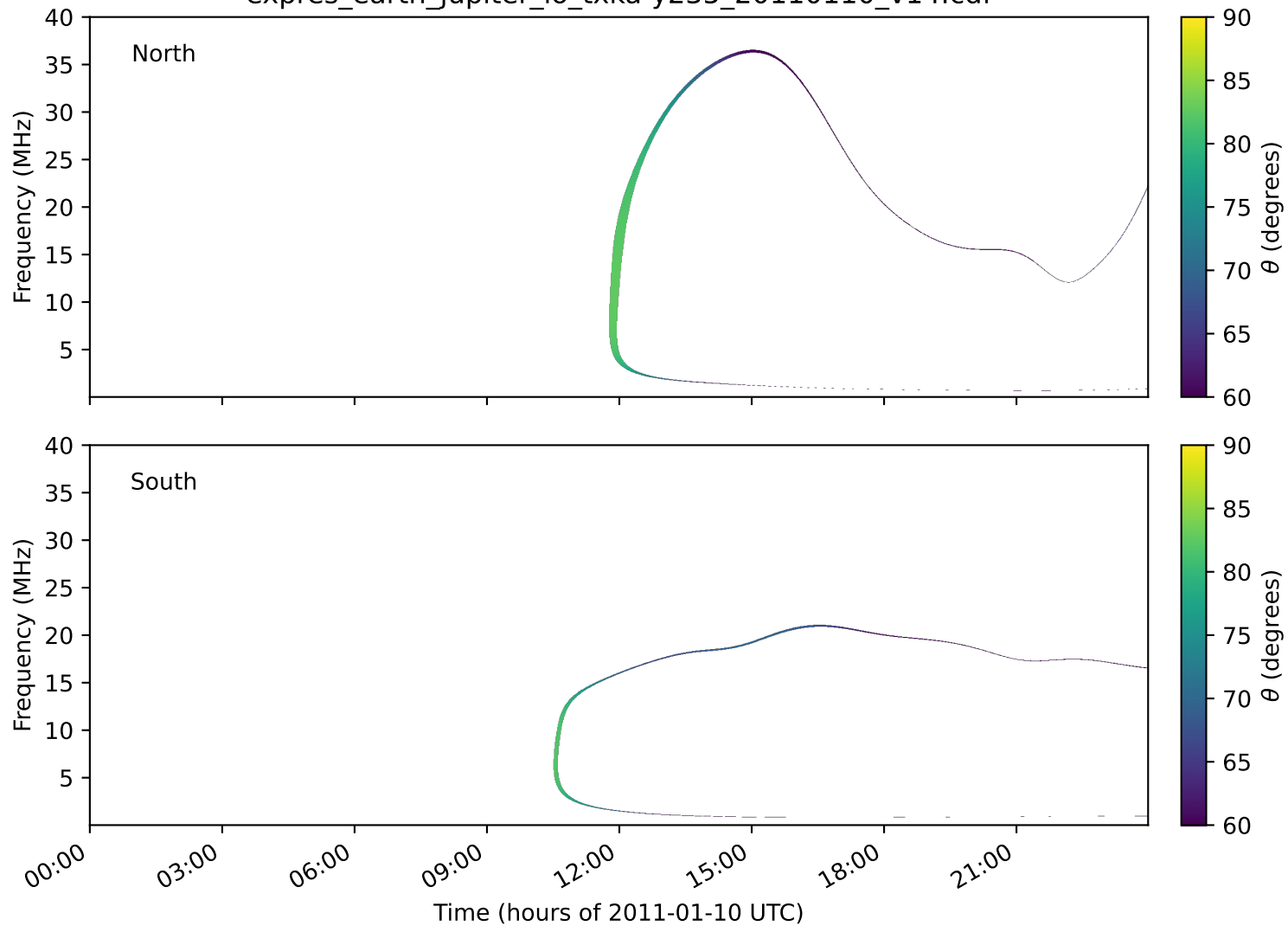
expres_earth_jupiter_io_txka-y235_20110110_v14.cdf
