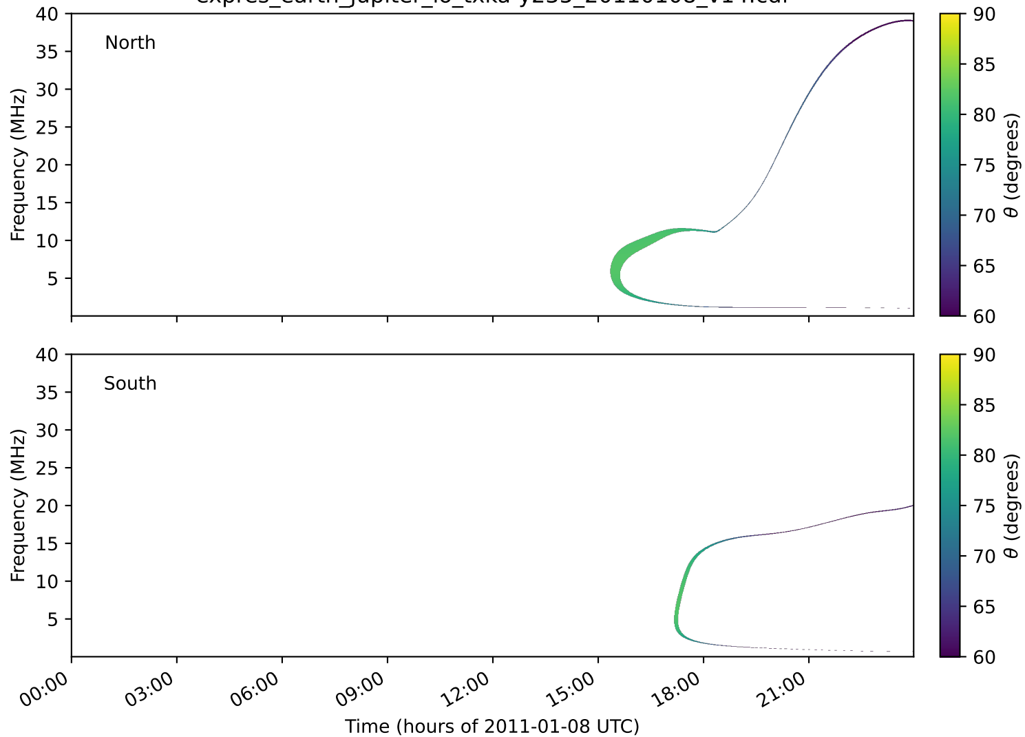
expres_earth_jupiter_io_txka-y235_20110108_v14.cdf
