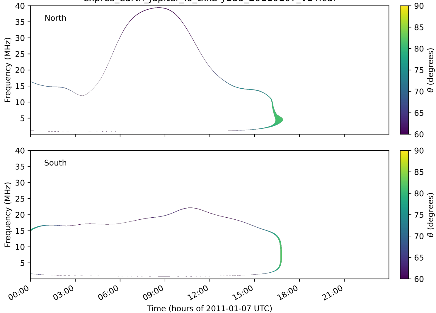
expres_earth_jupiter_io_txka-y235_20110107_v14.cdf
