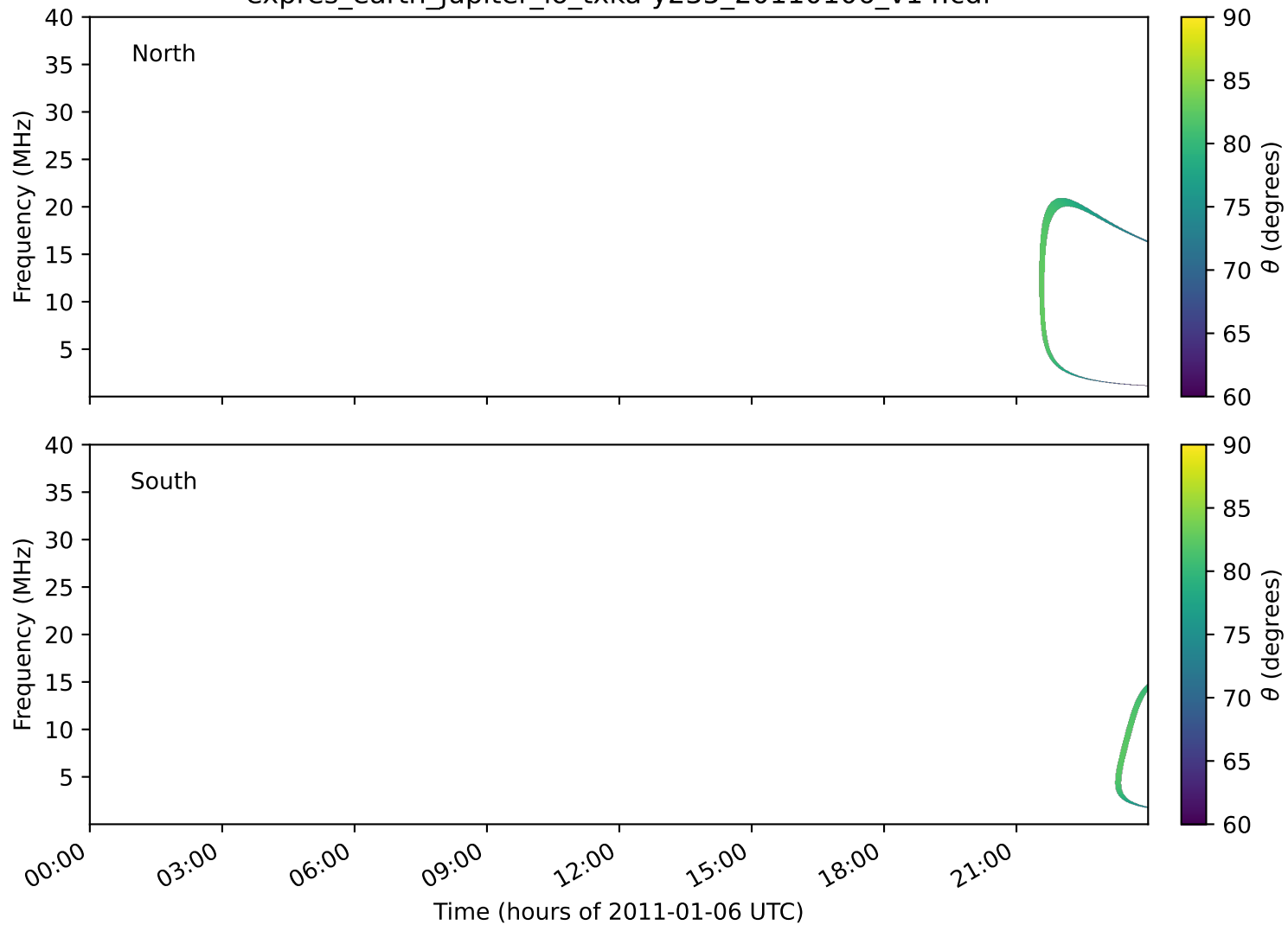
expres_earth_jupiter_io_txka-y235_20110106_v14.cdf
