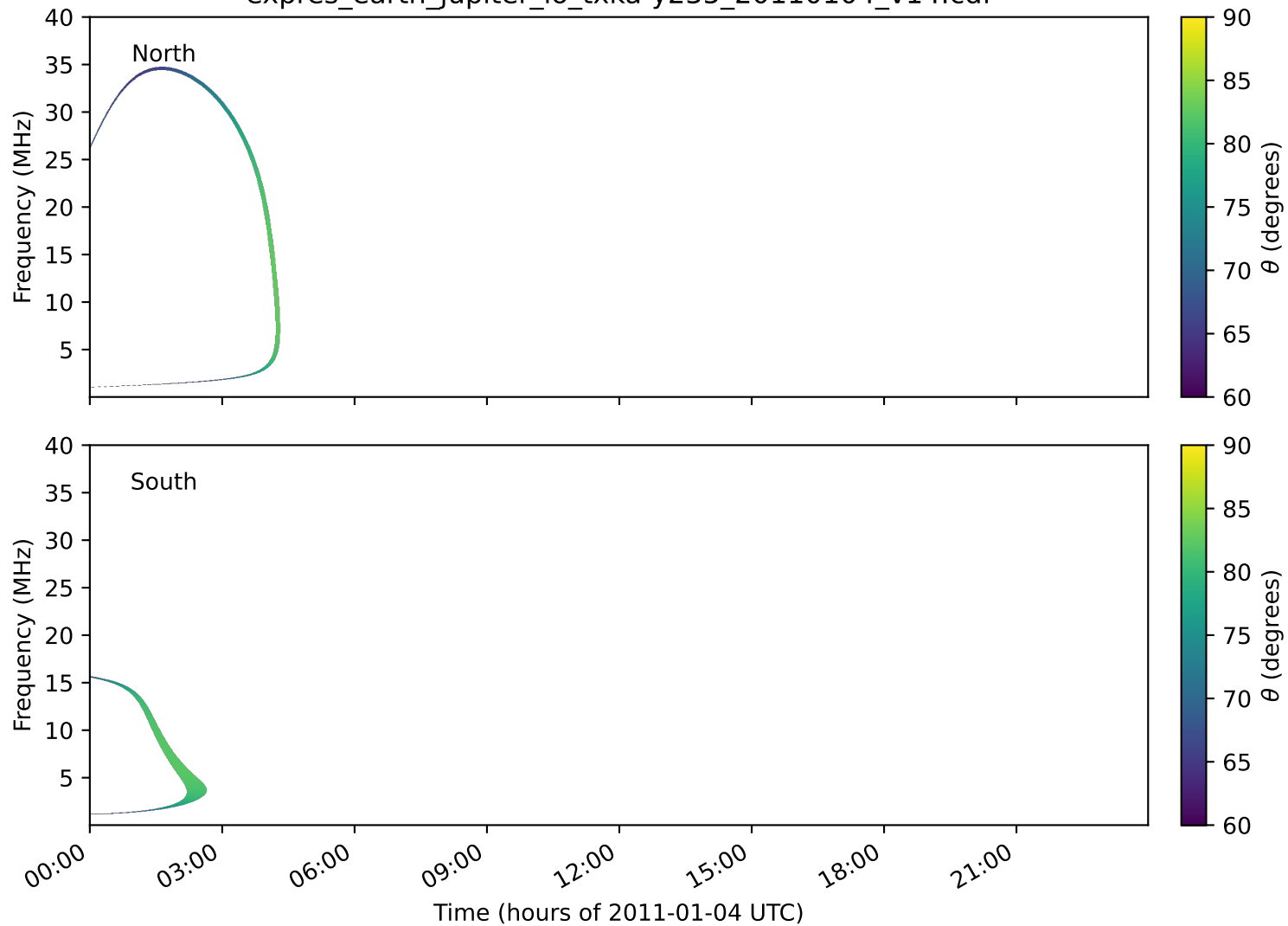
expres_earth_jupiter_io_txka-y235_20110104_v14.cdf
