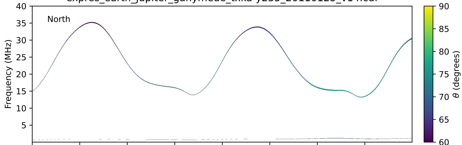
expres_earth_jupiter_ganymede_txka-y235_20110125_v14.cdf
