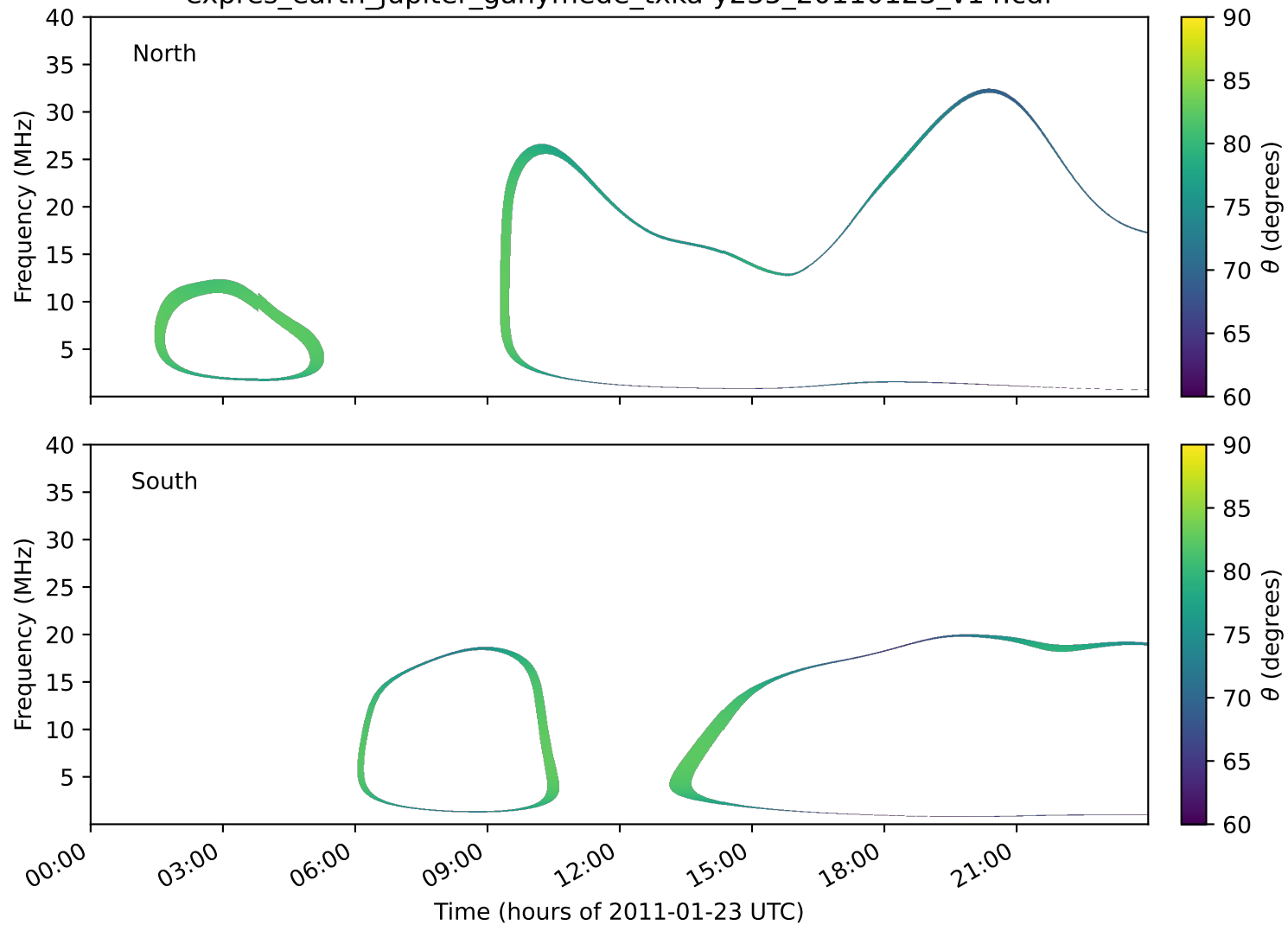
expres_earth_jupiter_ganymede_txka-y235_20110123_v14.cdf
