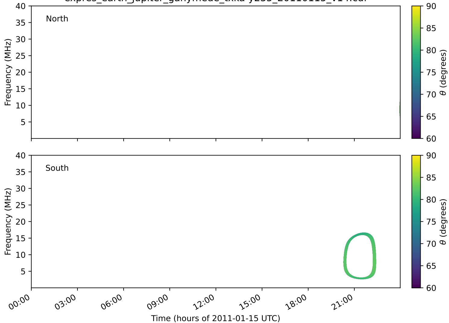
expres_earth_jupiter_ganymede_txka-y235_20110115_v14.cdf
