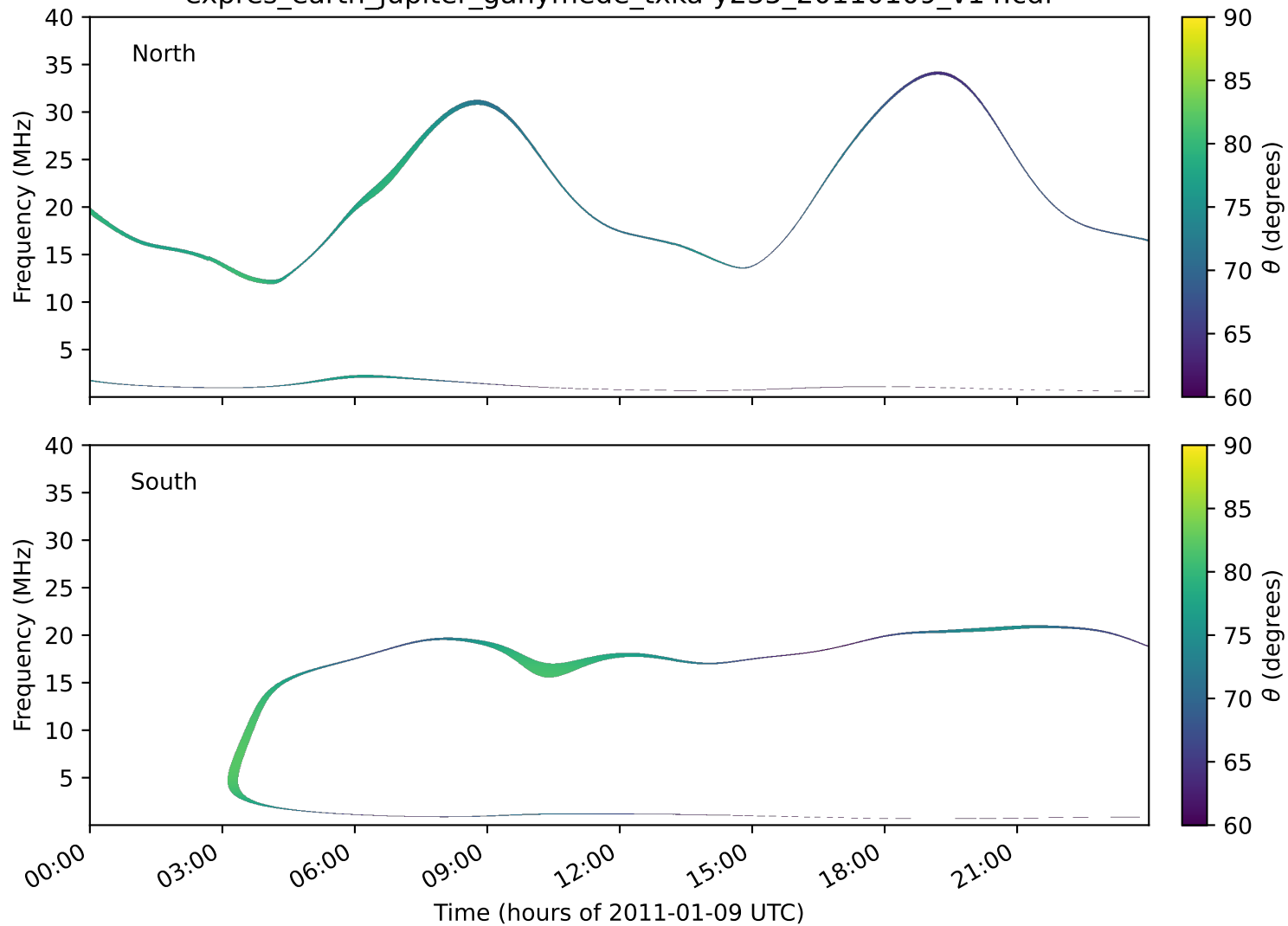
expres_earth_jupiter_ganymede_txka-y235_20110109_v14.cdf
