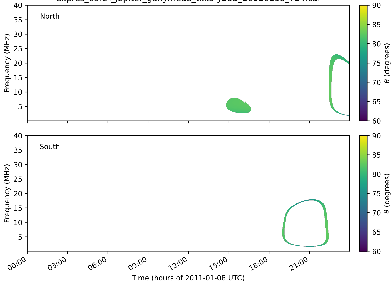
expres_earth_jupiter_ganymede_txka-y235_20110108_v14.cdf
