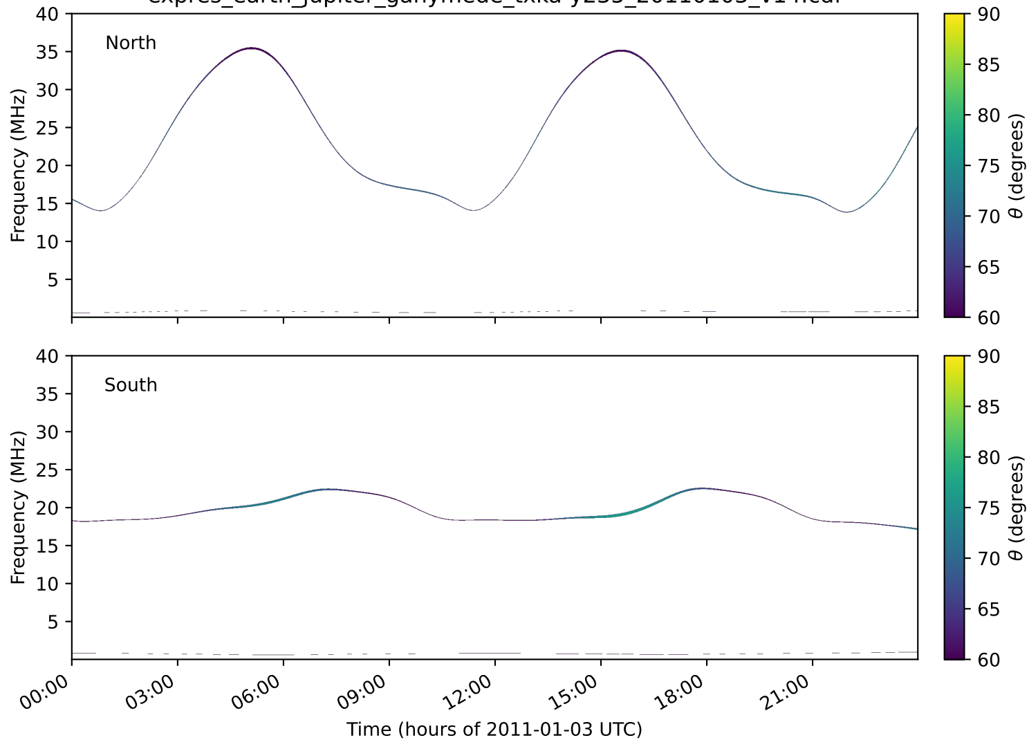
expres_earth_jupiter_ganymede_txka-y235_20110103_v14.cdf
