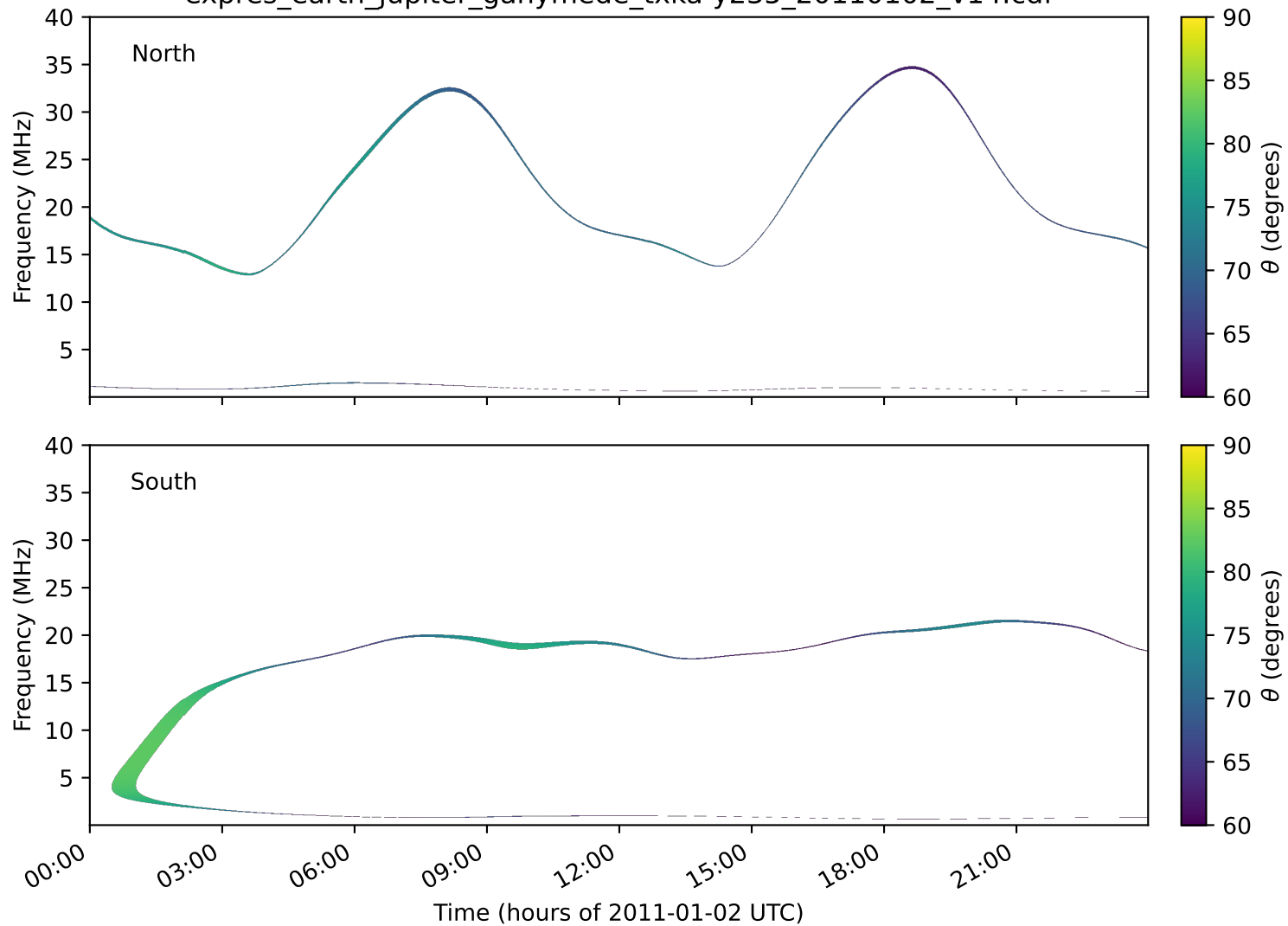
expres_earth_jupiter_ganymede_txka-y235_20110102_v14.cdf
