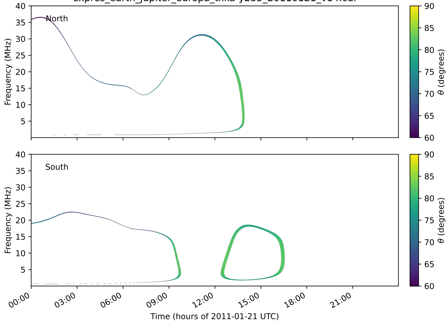
expres_earth_jupiter_europa_txka-y235_20110121_v14.cdf
