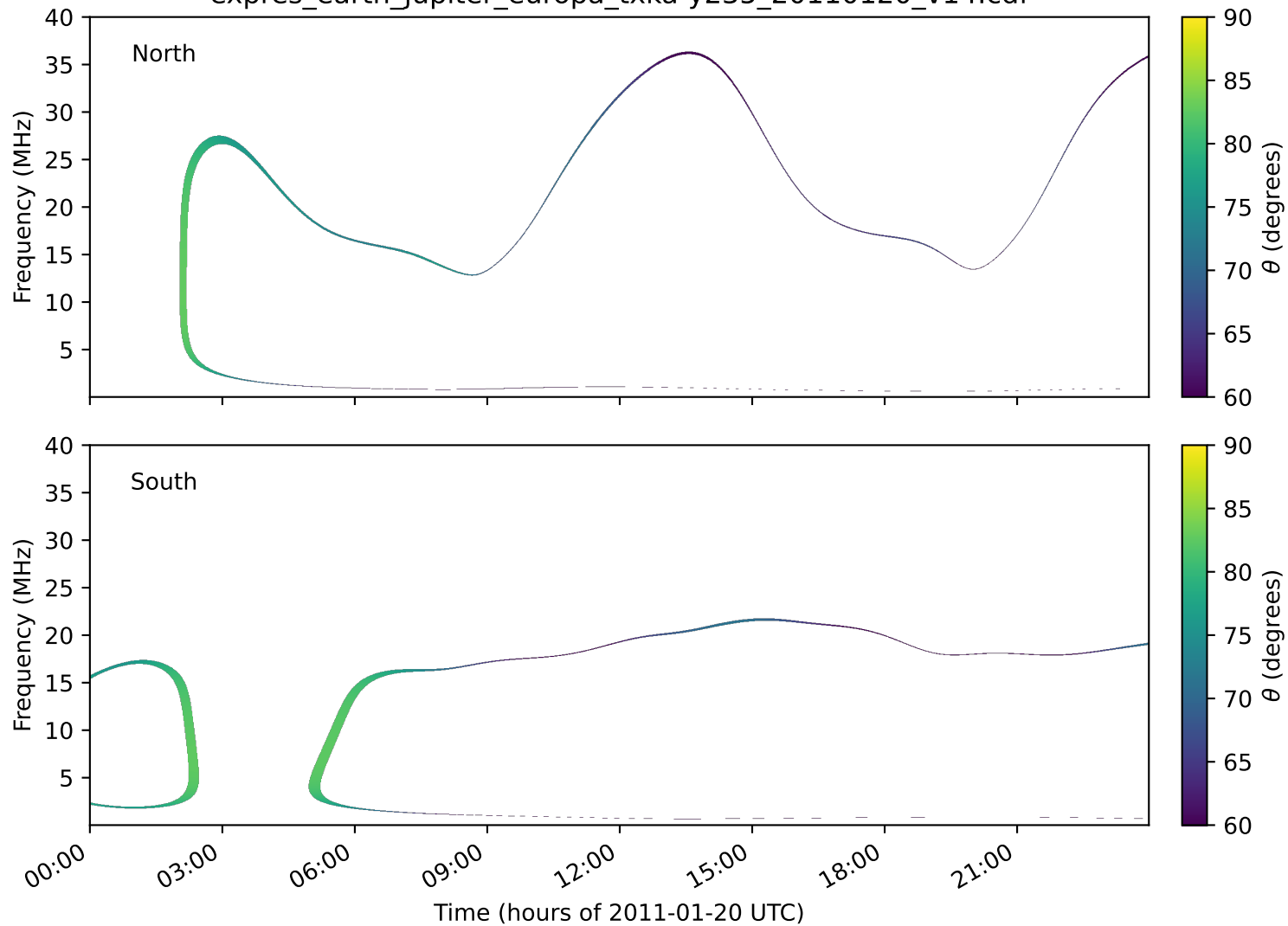
expres_earth_jupiter_europa_txka-y235_20110120_v14.cdf
