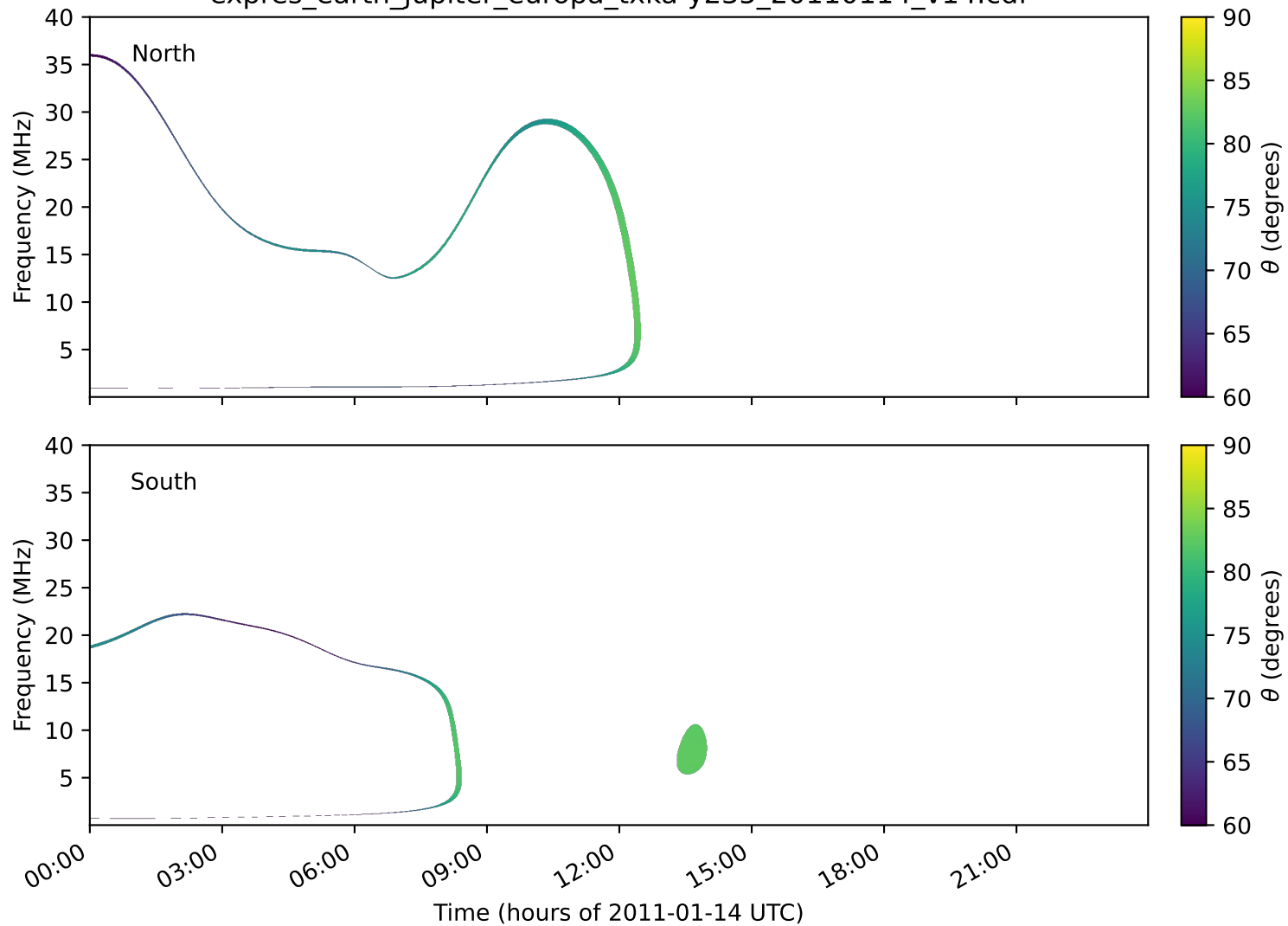
expres_earth_jupiter_europa_txka-y235_20110114_v14.cdf
