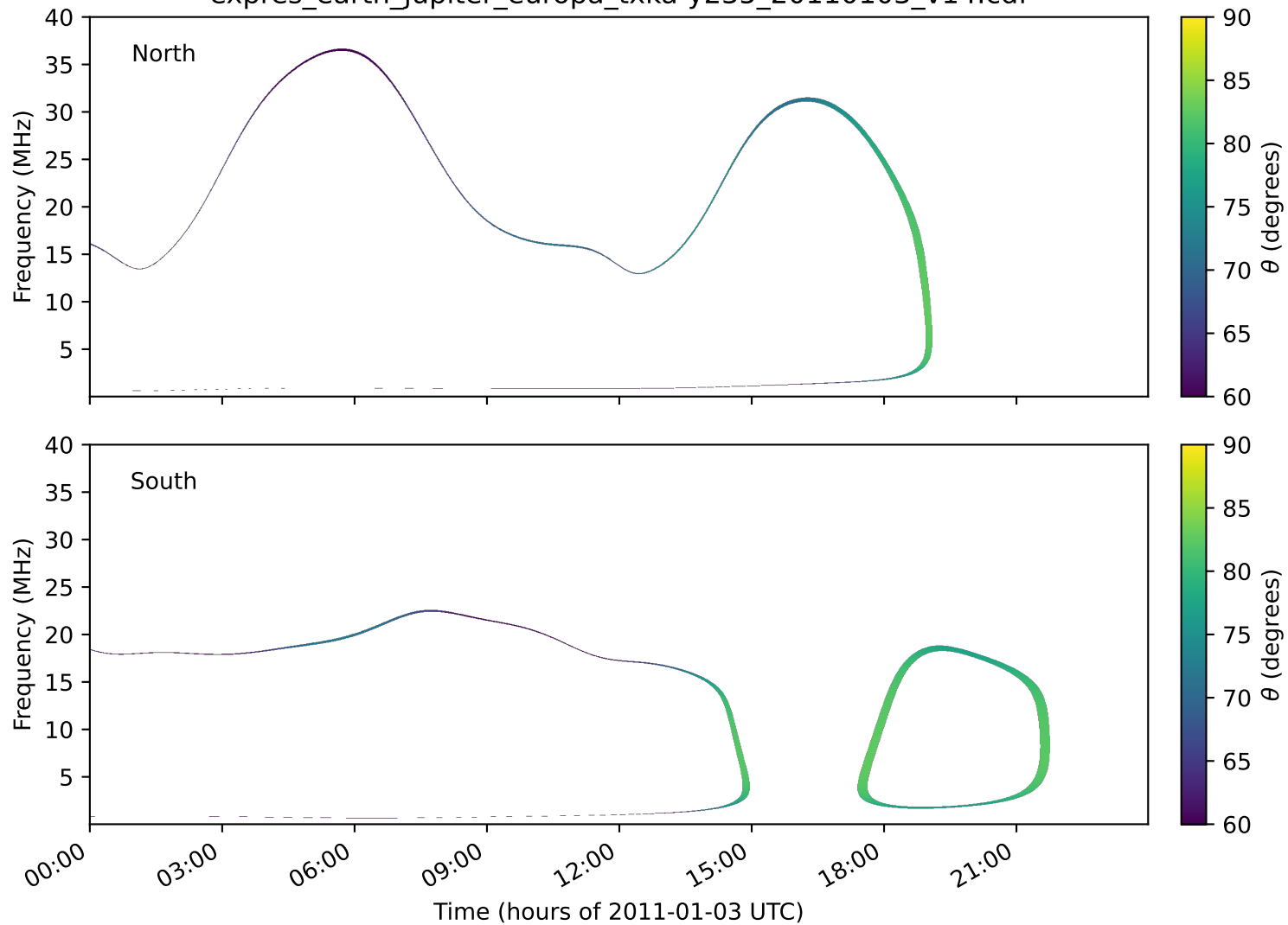
expres_earth_jupiter_europa_txka-y235_20110103_v14.cdf
