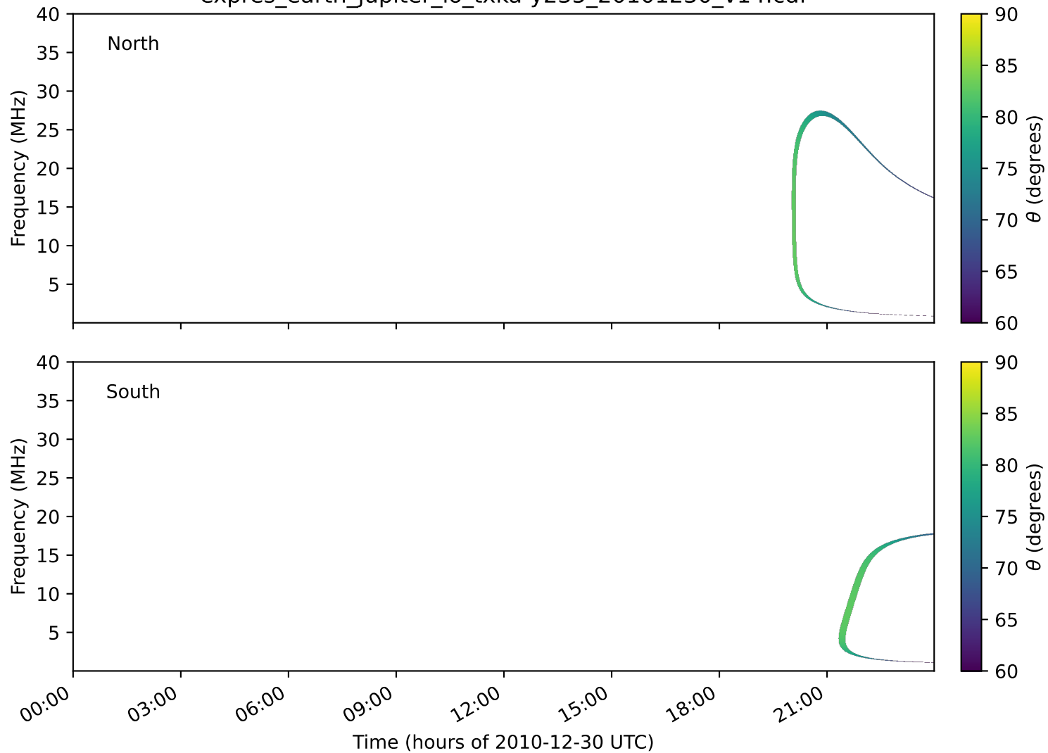
expres_earth_jupiter_io_txka-y235_20101230_v14.cdf
