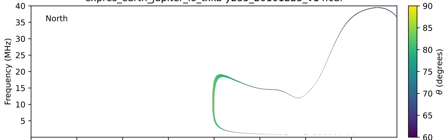
expres_earth_jupiter_io_txka-y235_20101225_v14.cdf
