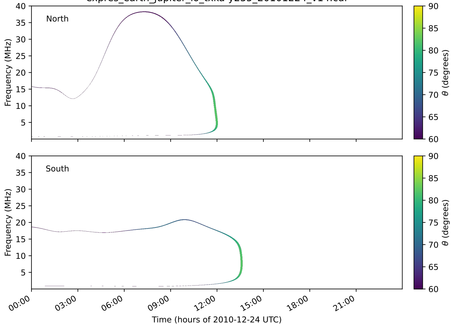
expres_earth_jupiter_io_txka-y235_20101224_v14.cdf
