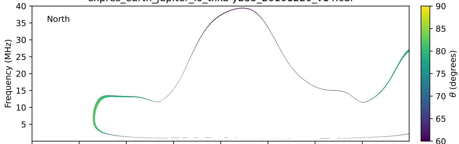
expres_earth_jupiter_io_txka-y235_20101220_v14.cdf
