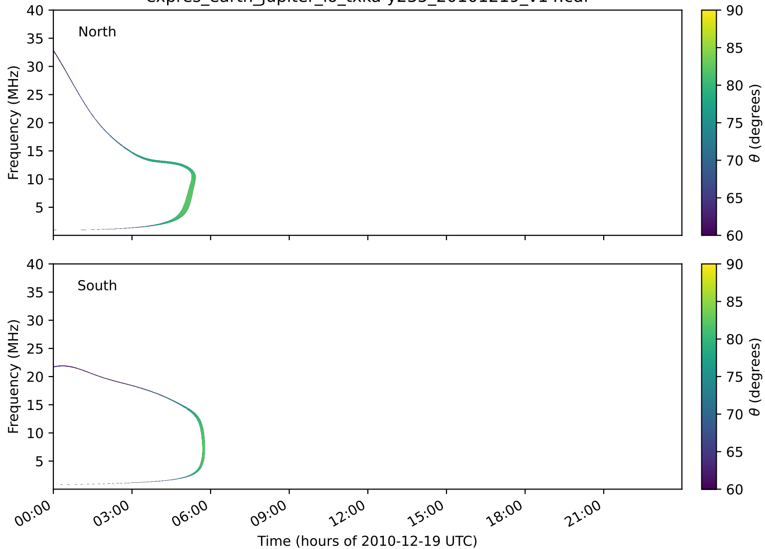
expres_earth_jupiter_io_txka-y235_20101219_v14.cdf
