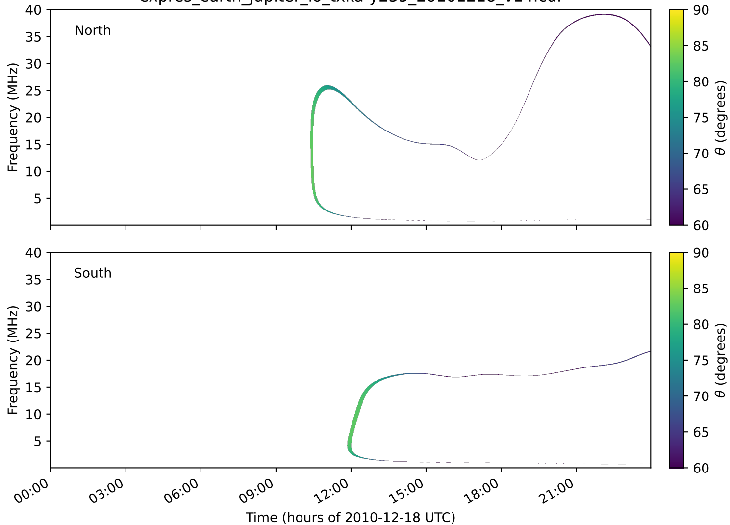
expres_earth_jupiter_io_txka-y235_20101218_v14.cdf
