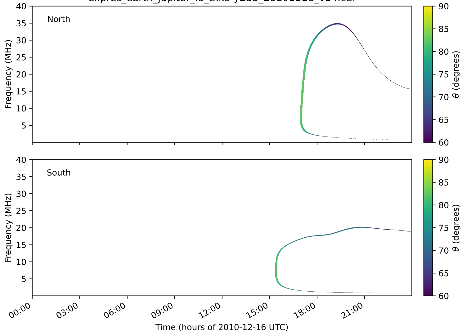
expres_earth_jupiter_io_txka-y235_20101216_v14.cdf
